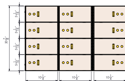
SS-4PV3 12 - 5 x 10 Stainless Steel Doors
